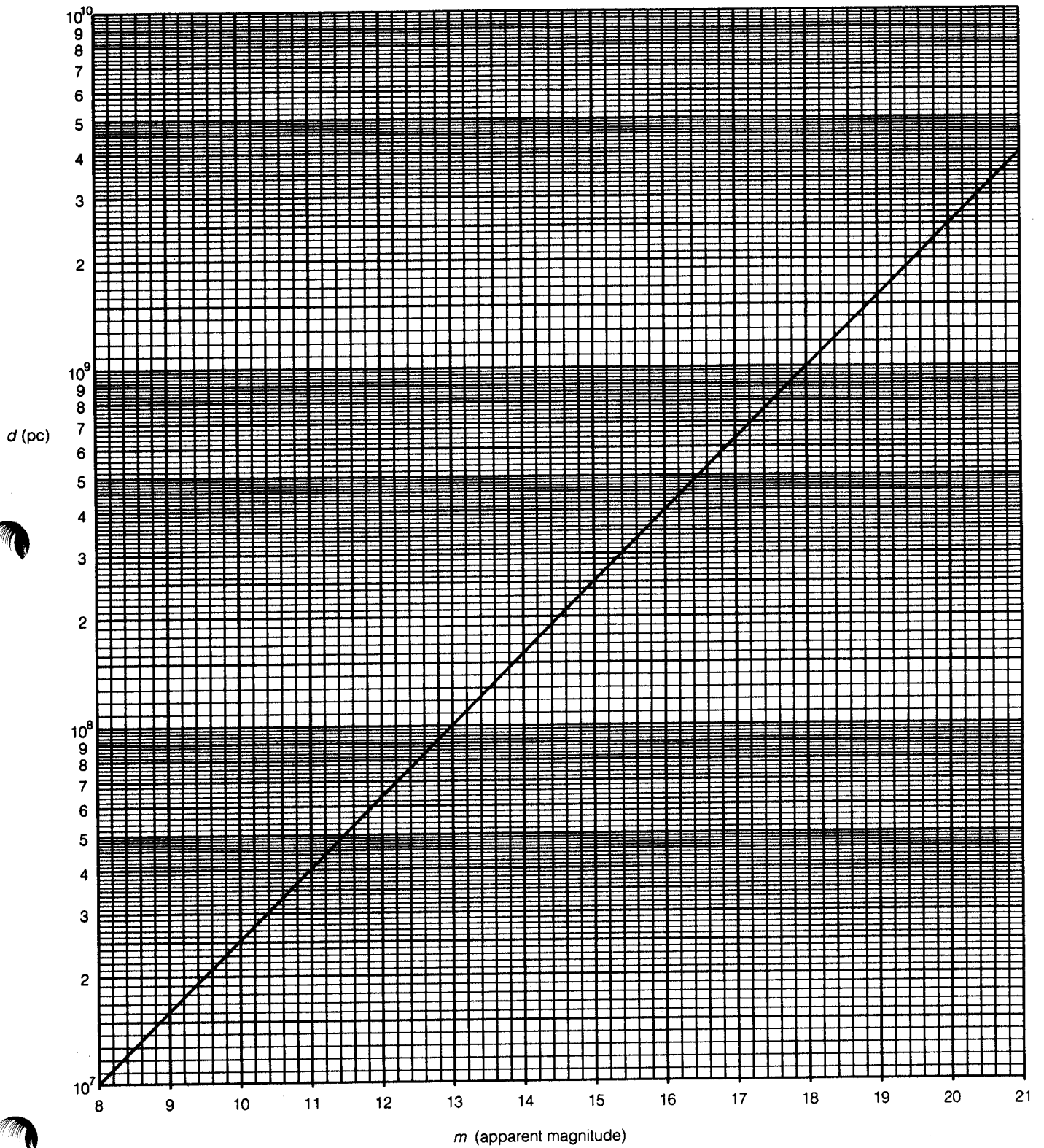
Figure 28.1 Relationship between d and m ( M = -22.0 ).
