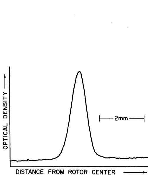
FIG. 7.—Microdensitometer tracing of an ultraviolet absorption photograph showing the optical density in the region of a band of N^{14} E. coli DNA at equilibrium. About 2 \mu g. of DNA purified as described in the text was centrifuged at 31,410 rpm at 25° in 7.75 molal CsCl at pH 8.4. The density gradient is essentially constant over the region of the band and is 0.057 gm./cm. 4 . The position of the maximum indicates a buoyant density of 1.71 gm. cm. -3 . In this tracing the optical density above the base line is directly proportional to the concentration of DNA in the rotating centrifuge cell. The concentration of DNA at the maximum is about 50 \mu g./ml.
