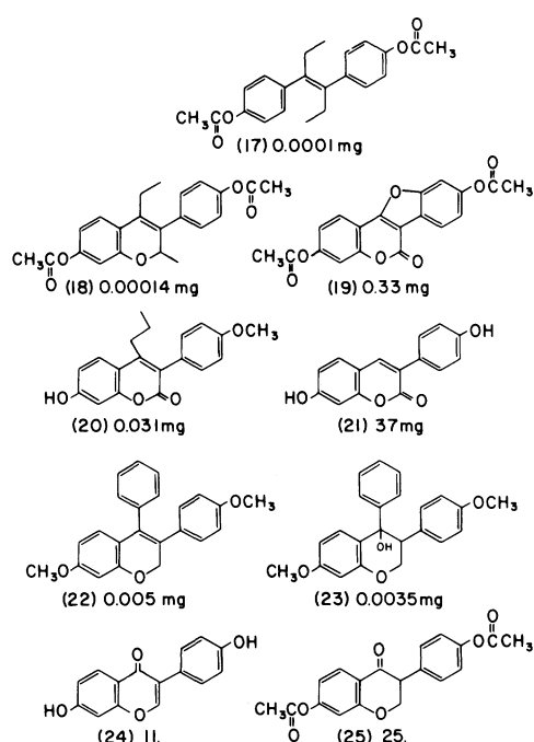
FIGURE 14. Structure-activity relationships of nonsteroidal estrogens related to phytoestrogens. The dose necessary to produce an increase of immature mouse uterine wet weight to 20 mg from a control value of 10 mg is shown for each compound (oral administration). Data adapted from Micheli et al. (92).
