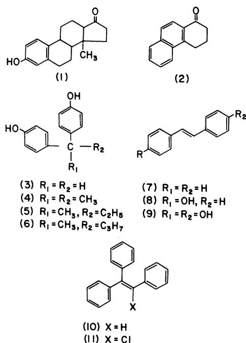
FIGURE 1. Formulae of compounds found, in the 1930s, to have estrogenic activity in vivo . Compound 1 was believed to be the molecular structure of ketohydroxyestrin (estrone). This is now known to be incorrect.
