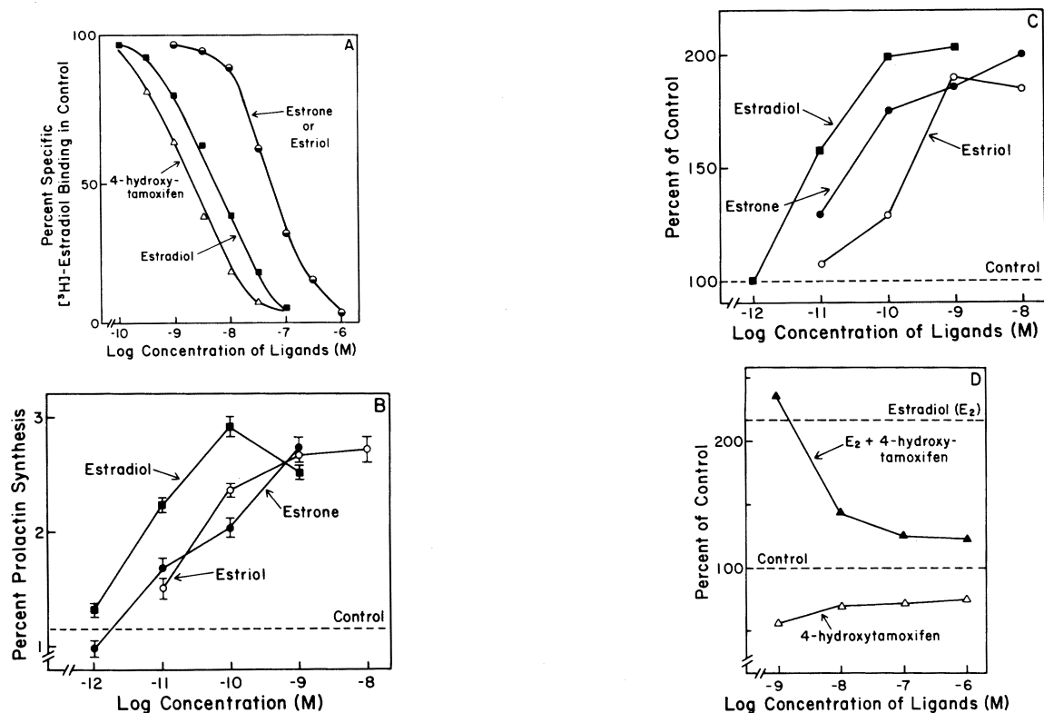
FIGURE 6. Receptor binding and biological activity in vitro of estradiol, estrone, estriol, and 4-hydroxytamoxifen: (A) inhibition of the binding of [ 3 H]estradiol to rat uterine estrogen receptors in vitro by 4-hydroxytamoxifen, estradiol, estrone, and estriol; (B) increase in the percent prolactin synthesis produced by the culture of dispersed cells from immature rat pituitary glands with increasing concentrations of estradiol, estriol, and estrone; (C) percent increase (over control) of progesterone receptor in cultures of dispersed cells from immature rat uteri with increasing concentrations of estradiol, estriol, and estrone; (D) percent decrease of estradiol (1 nM)-stimulated progesterone receptor in cultures of dispersed cells from immature rat uteri produced by increasing concentrations of 4-hydroxytamoxifen.
