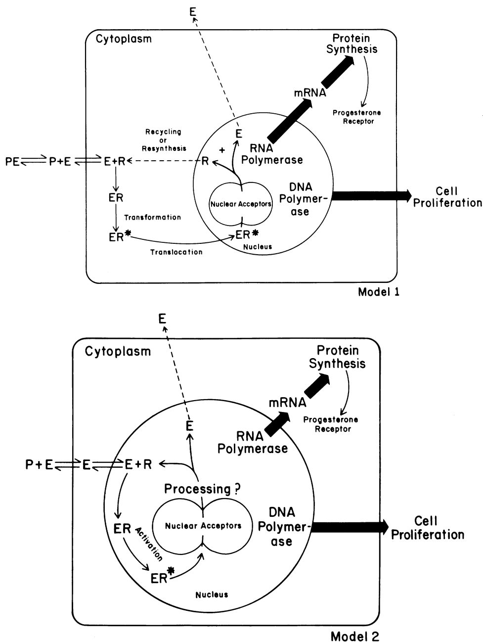
FIGURE 3. Subcellular models of estrogen action. Estrogen (E) dissociates from plasma proteins (P) and diffuses into the target cell. In Model 1 the receptor (R) is located in the cytoplasm and in Model 2 the receptor is in the nuclear compartment. In both models the receptor complex is activated before initiating protein synthesis and finally cell division. The fate of the receptor is at present unknown; it may be recycled, destroyed (processed) or resynthesized.
