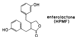
FIGURE 8. Formula of enterolactone which has also been referred to as HPMF (65).
