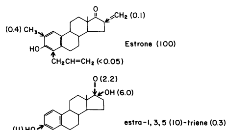
FIGURE 12. Structure-activity relationships of estrone. The structure-activity relationships of steroids in the 3-day immature mouse uterine weight test using estrone as the standard. The relative potencies are shown in parentheses using estrone equivalent to 100. Data adapted from Dorfman and Kincl (88).
