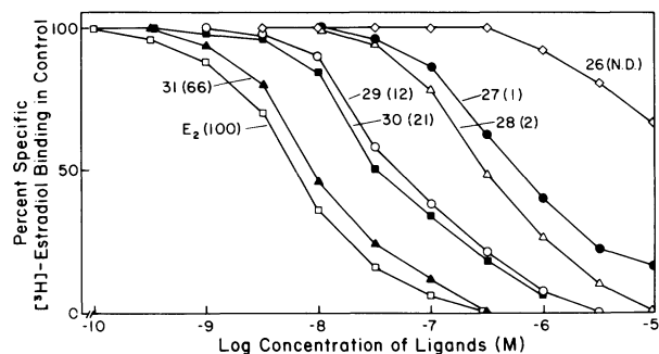
FIGURE 17. Inhibition of the binding of [ ^3\text{H} ]estradiol to rat uterine estrogen receptors in vitro by different substituted triphenylethylenes described in Fig. 15. The assay was conducted at 4°C and incubation was for 18 hr. The RBAs in parentheses are calculated as [(M) concn \text{E}_2 for 50% inhibition]/[(M) concn competitor for 50% inhibition] \times 100.
