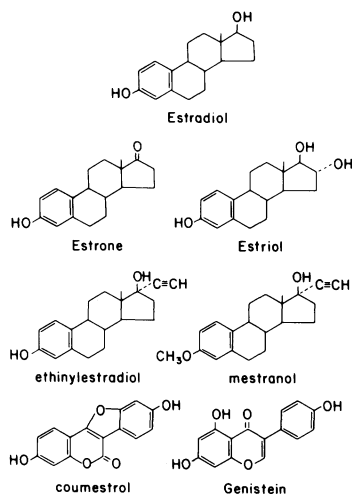
FIGURE 4. Formulae of some steroidal estrogens and the phytoestrogens coumestrol and genistein.
