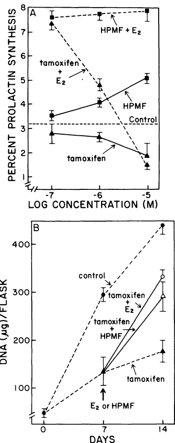
FIGURE 9. Biological activity of HPMF: (A) Inhibition of estradiol (1 nM)-stimulated prolactin synthesis by tamoxifen. HPMF did not inhibit estradiol-stimulated prolactin synthesis but 10 \mu\text{M} stimulated prolactin synthesis in immature rat pituitary cells in culture. (B) Inhibition of the growth of MCF7 breast cancer cells by tamoxifen (1 \mu\text{M} ). Estradiol (10 nM) or HPMF (10 \mu\text{M} ) reversed the effect of tamoxifen on cell growth.
