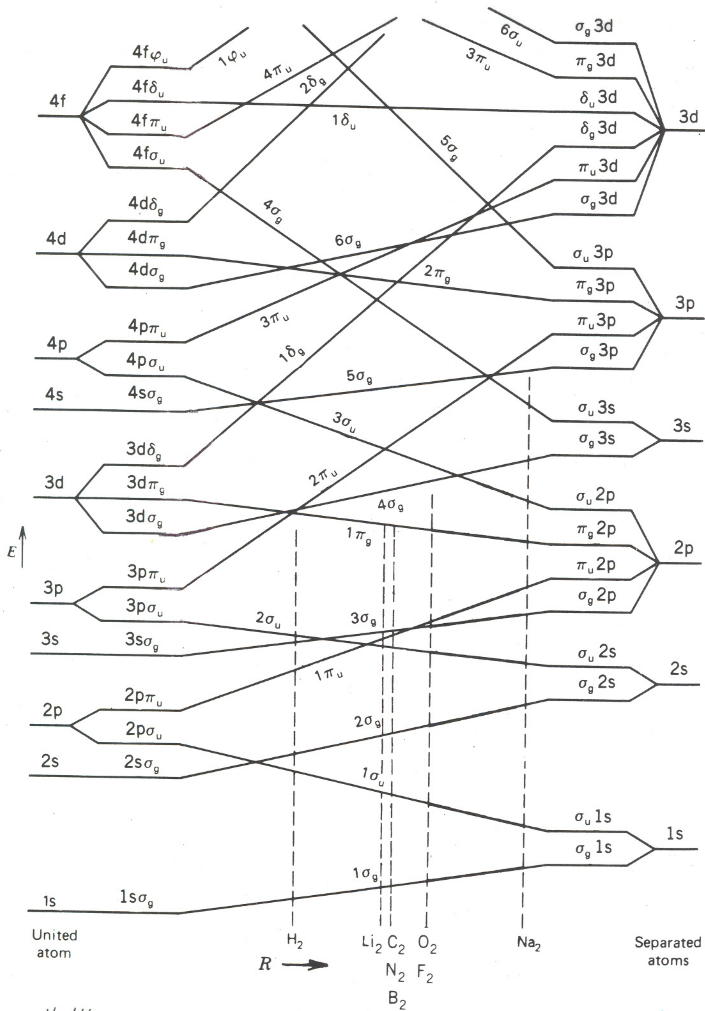
11.14 Figure 12.13 Correlation diagram for homonuclear diatomic molecules. The energy scale is schematic, but dashed lines show the correct sequence for filling of orbitals for the molecules indicated. (From R. S. Berry, S. A. Rice, and J. Ross, Physical Chemistry . New York: Wiley, 1980.)
